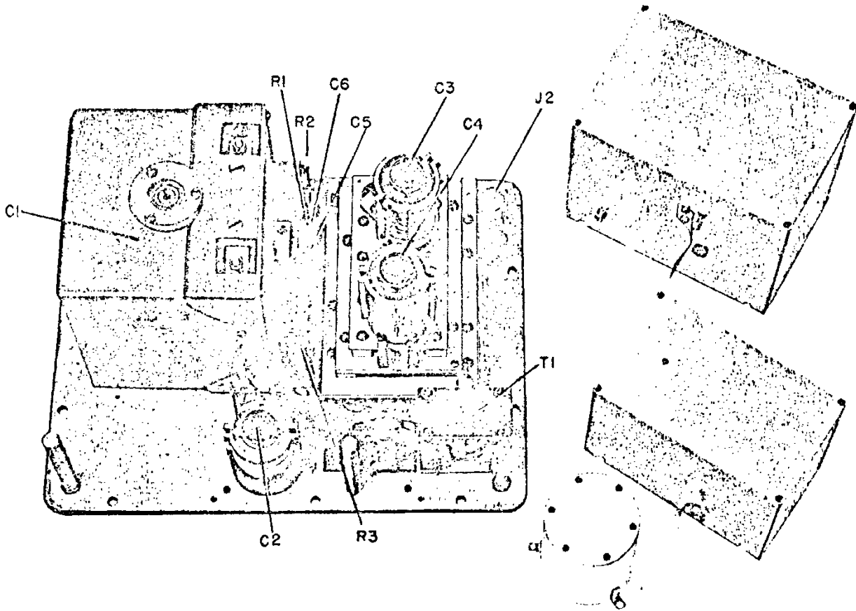
Figure 9. Interior View of Type 1606-A R-F Bridge.
