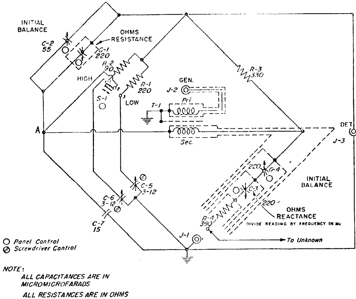
Figure 10. Schematic Diagram of Type 1606-A R-F Bridge.
