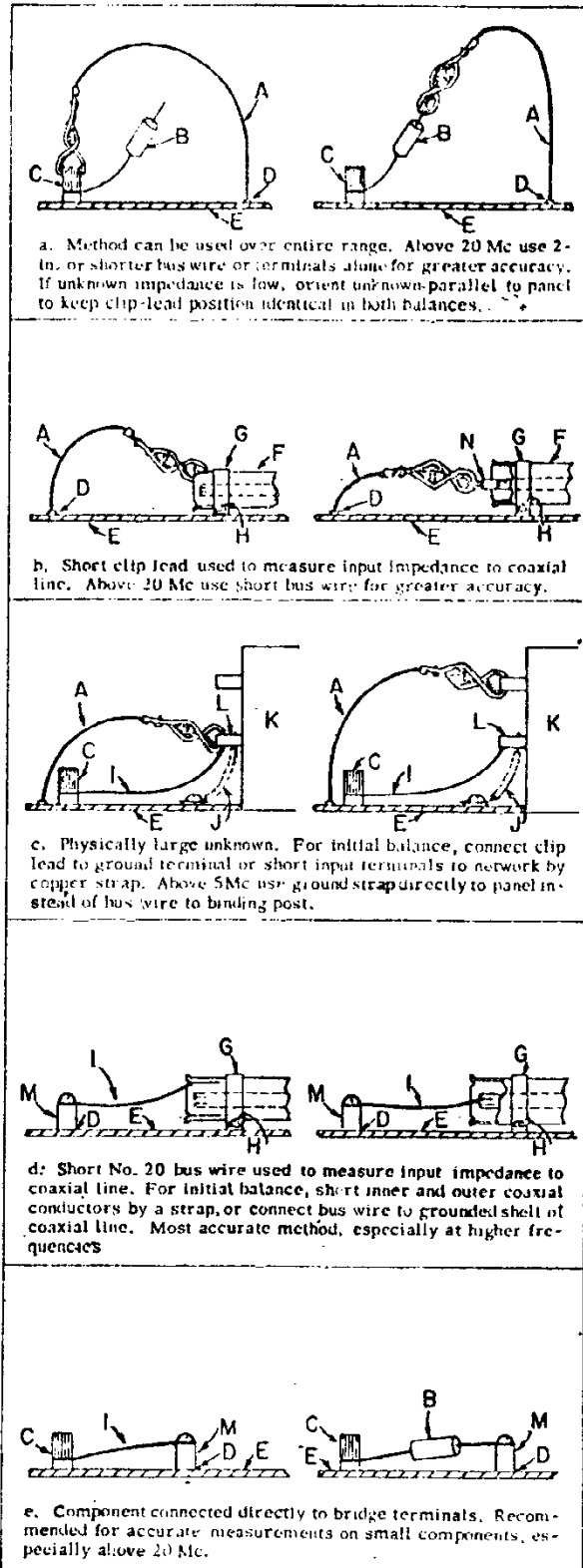
Figure 4. Methods of Connection.
